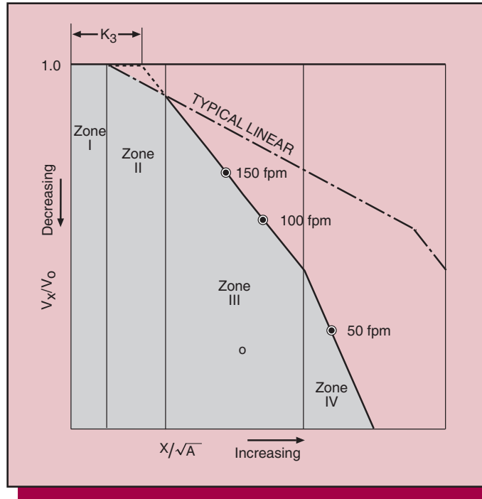
Figure 7. Four Zones of Expansion of Primary Air Jet
