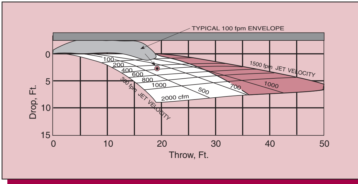
Figure 14. Throw and Drop for Outlet 1-½ Feet Below Ceiling, 0 Degree Vertical, 45 Degree Spread
