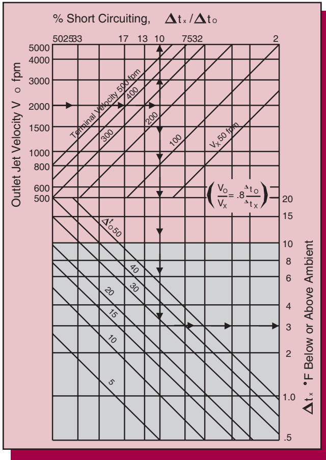
Figure 39. Temperature Differential and Short Circuiting
