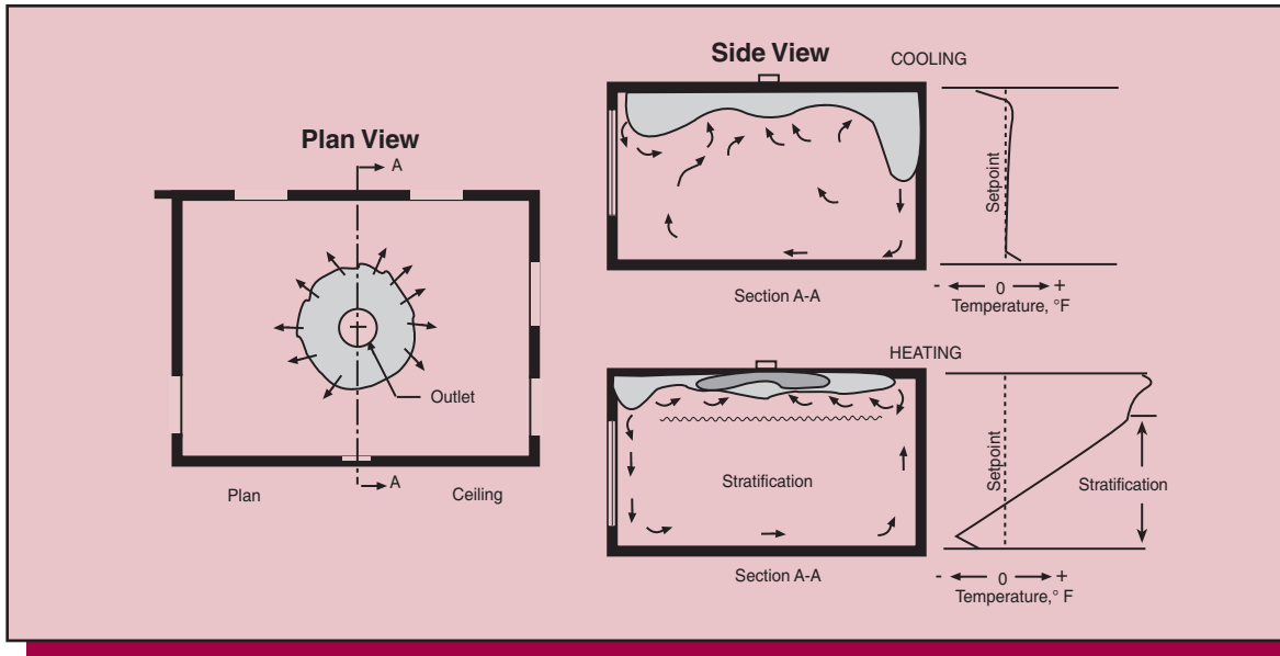
Figure 18. Circular Horizontal Air Projection at the Ceiling Level
