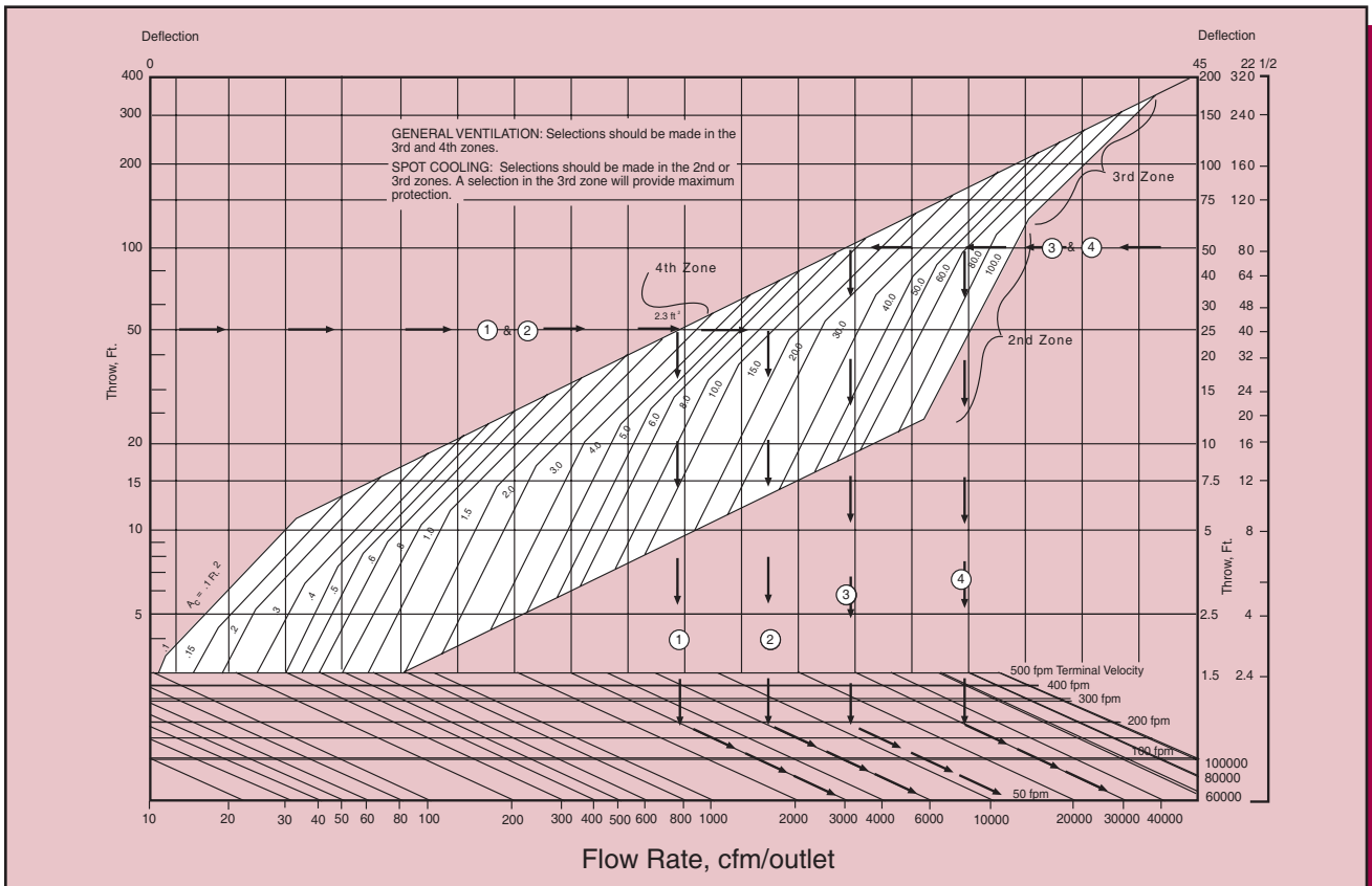
Figure 41. Grille Selection Chart for Industrial Applications
