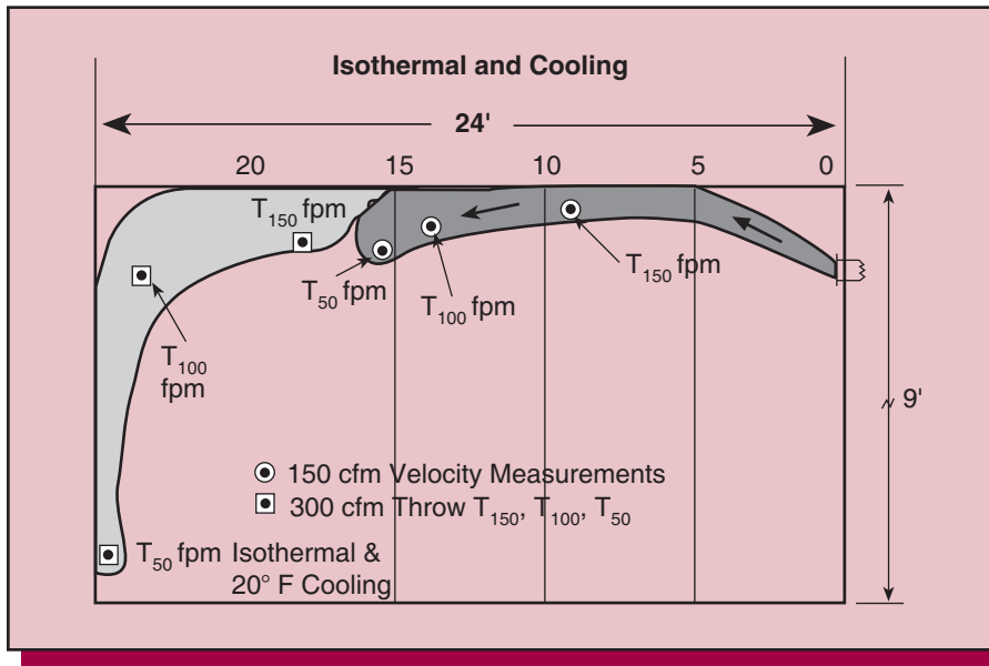
Figure 9. Mapping of Cooled Air Throw
