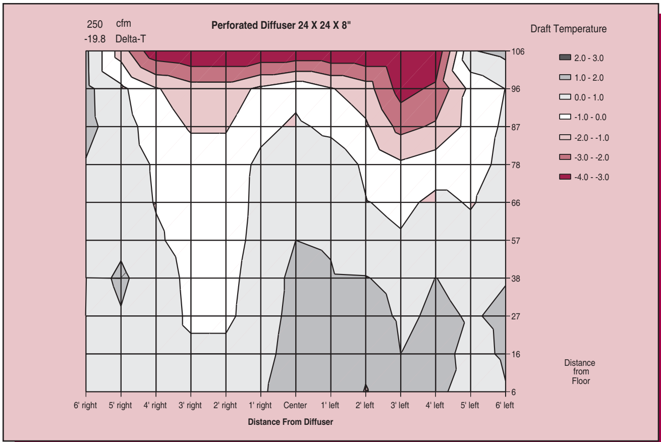
Figure 37. Room Isodrafts
