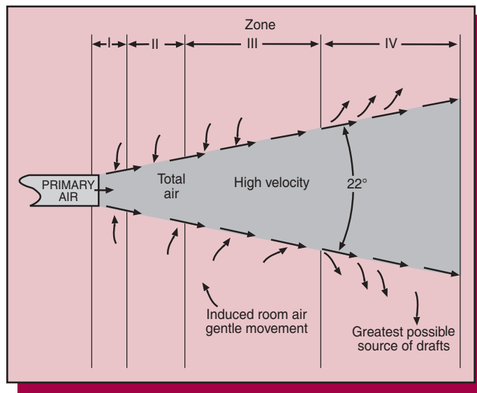
Figure 6. Expansion of primary air jet
