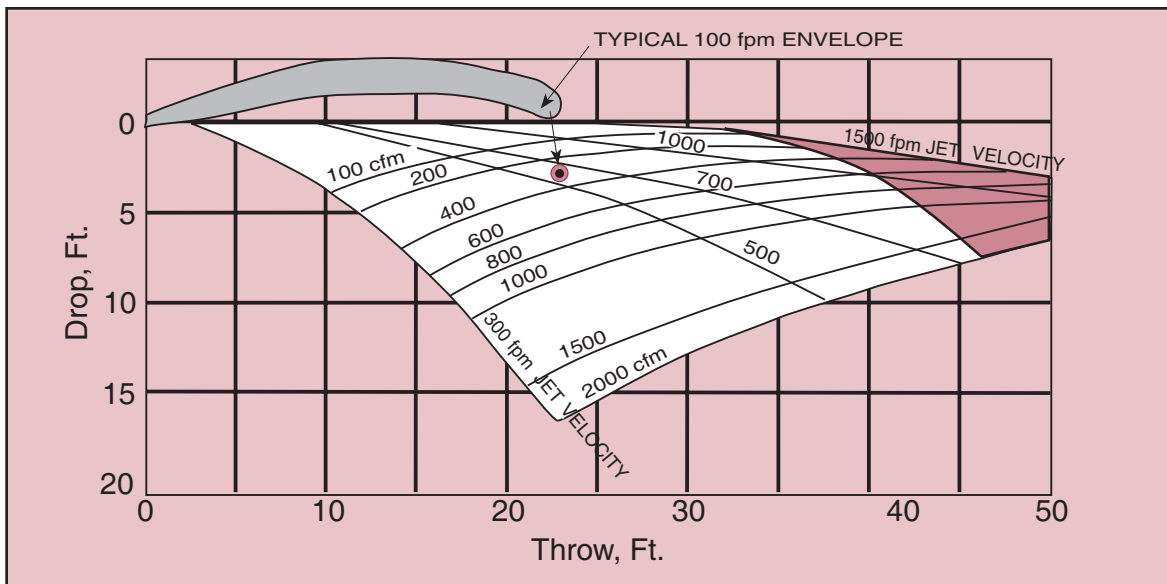
Figure 11. Throwing and Drop for Outlets Mounted Without Ceiling, 20 Degree Vertical Deflection, 0 Degree Spread
