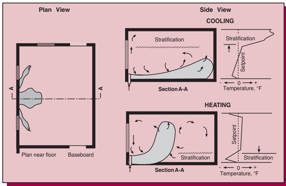
Figure 28. Horizontal Projection Spread at Floor Level
