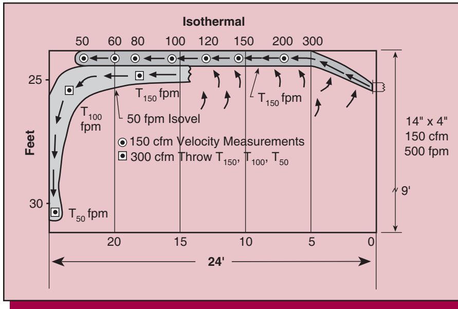
Figure 8. Mapping of Isothermal Throw
