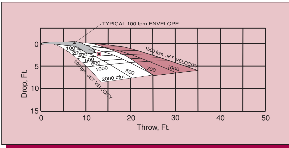
Figure 15. Throw and Drop for Outlet 2 to 4 Feet Below Ceiling, 0 Degree Vertical, 45 Degree Spread
