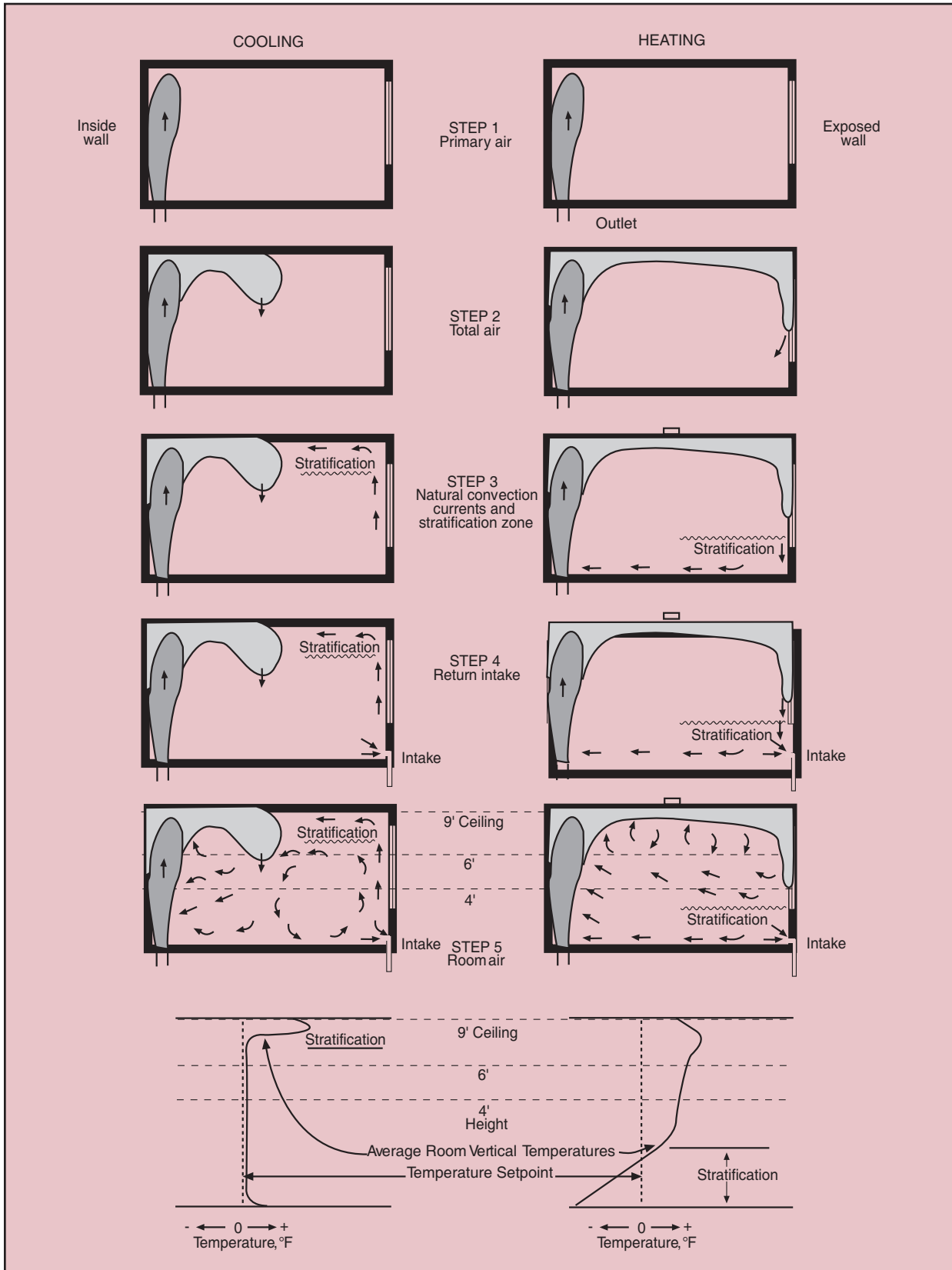
Figure 16. Characteristic of Non-isothermal Supply Jets in a Space
