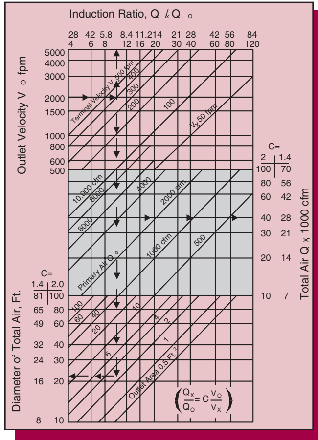
Figure 40. Induction Ratio, Total Air and Total Air Diameter
