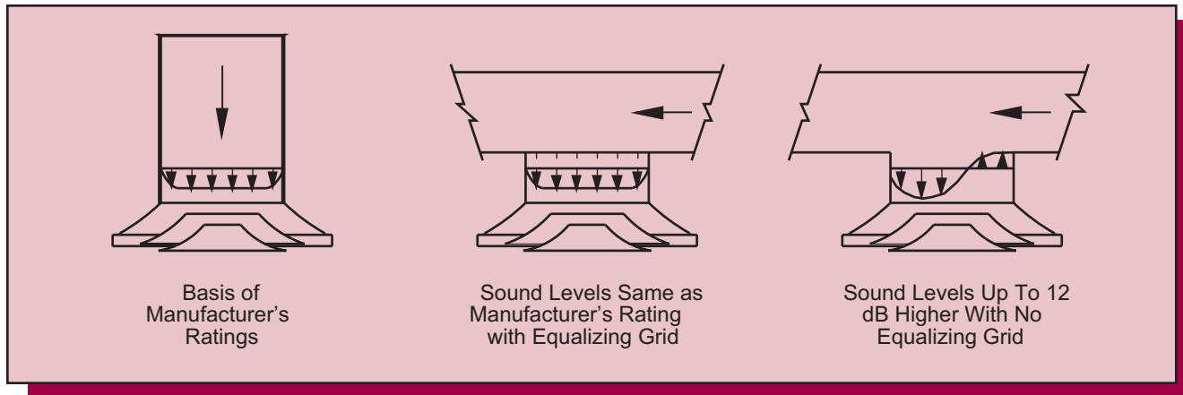
Figure 45. Equalizing Grid Effects (from ASHRAE Standards Handbook; Atlanta, GA)
