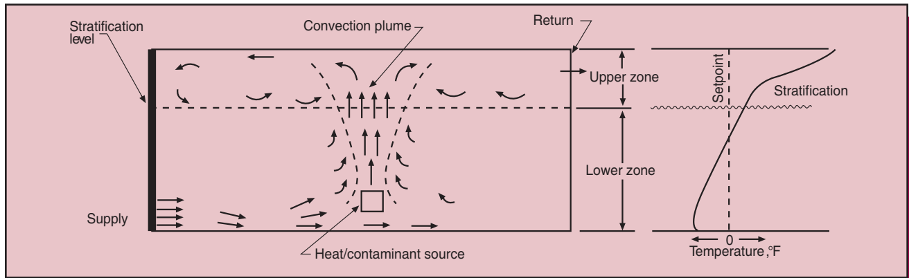
Figure 29. Spreading Upward Projection of Primary Air in the Stagnant Zone, Relatively Large Temperature Variations Occur
