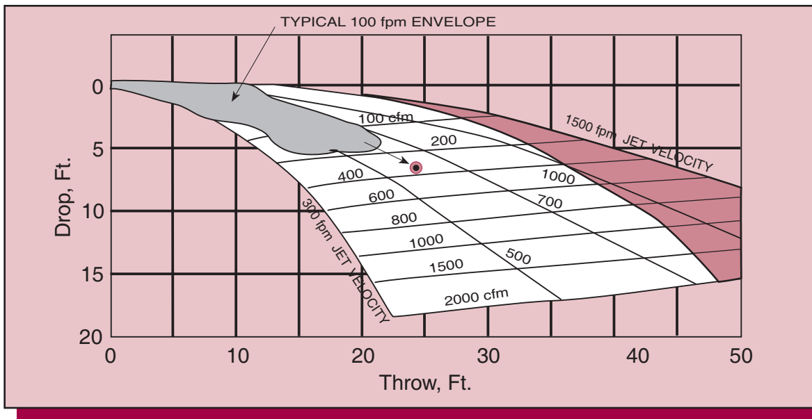
Figure 13. Throw and Drop for Outlet Without Ceiling, 0 Degree Deflection, 0 Degree Spread
