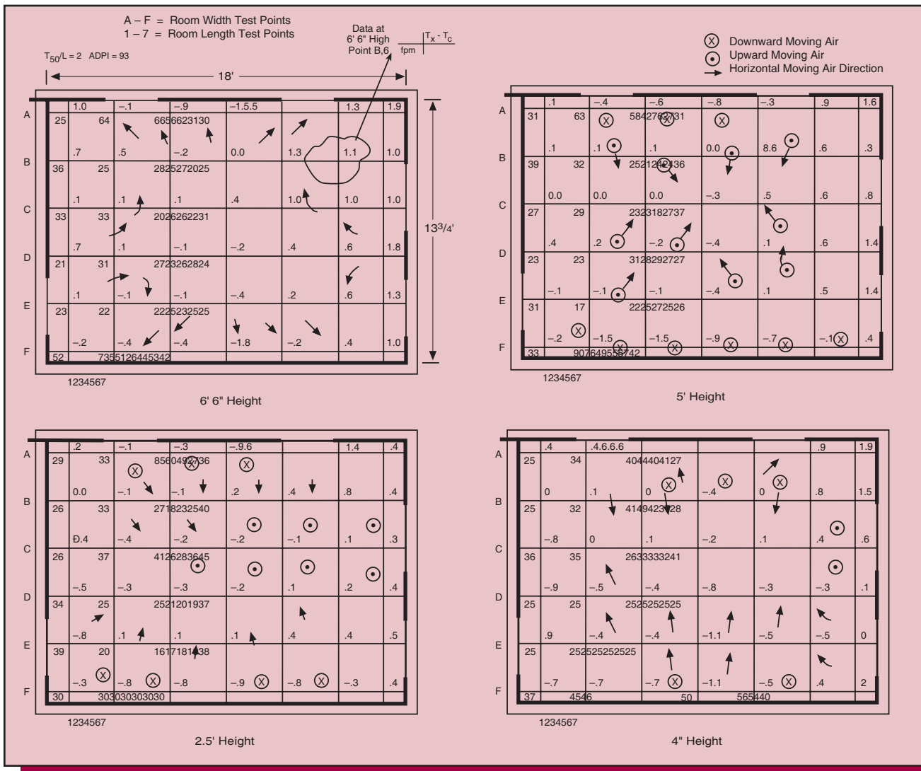
Figure 28. Horizontal Projection Spread at Floor Level
