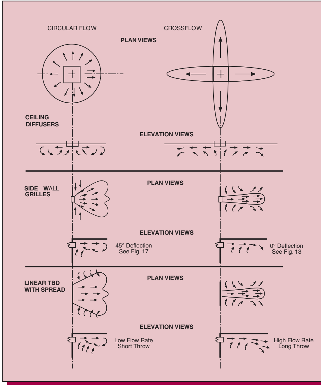
Figure 19. Some Specific Airflow Characteristics at High and Low Airflow Rates
