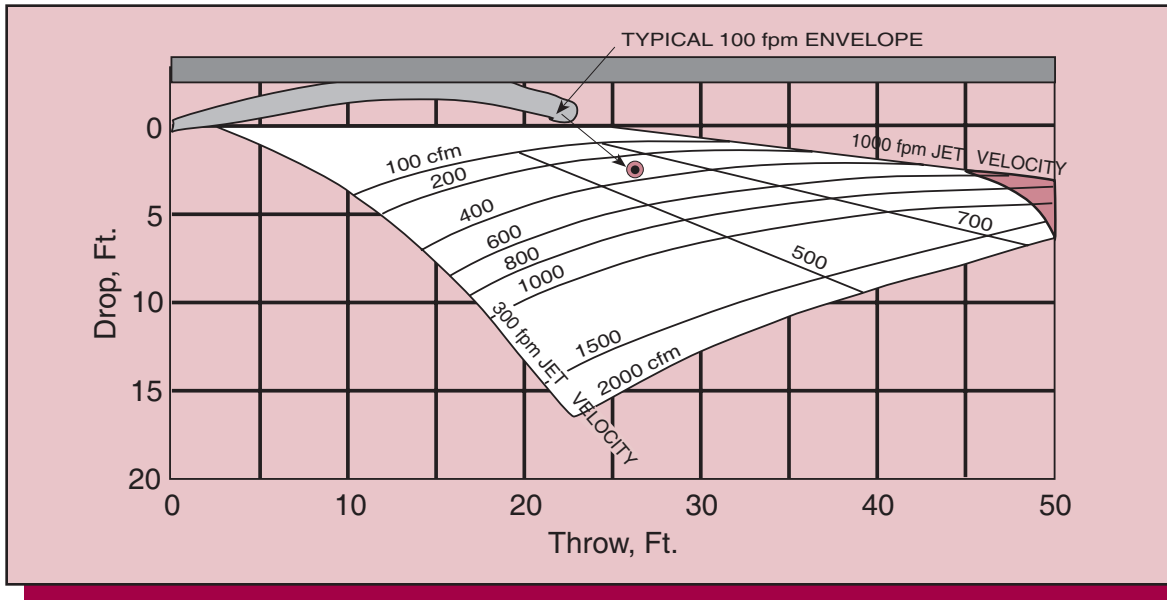
Figure 10. Throw and Drop for Outlet 2-4 feet Below Ceiling, 20 Degrees Vertical Deflection, 0 Degrees Spread
