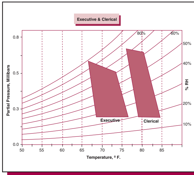
Figure 4. PMV Chart
