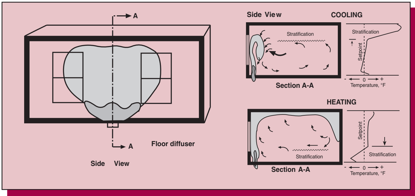
Figure 29. Spreading Upward Projection of Primary Air in the Stagnant Zone, Relatively Large Temperature Variations Occur
