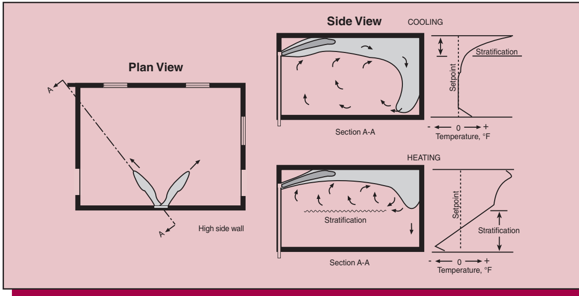
Figure 17. Spreading Horizontal Air Projection at the Ceiling Level
